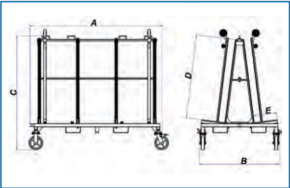
Large forklift slots to easily work combined with various forklift sizes
