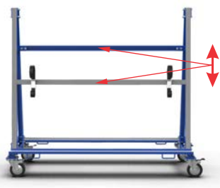
Crossbar can be adjusted upward or downward for flexible handling various slab sizes.
