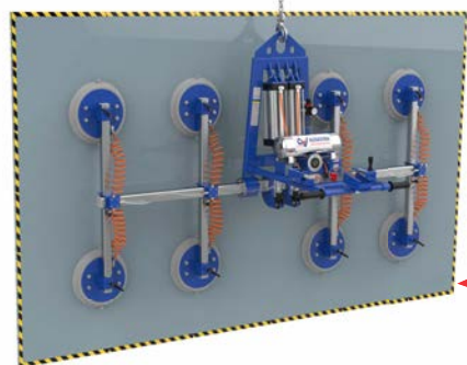
FLEXIBLE TILT FROM 0° TO 90°
