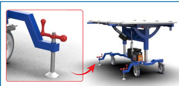
Support bars
